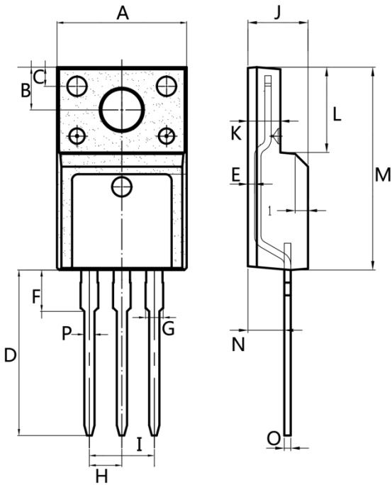
TO-220FAC 封装尺寸 Package size
