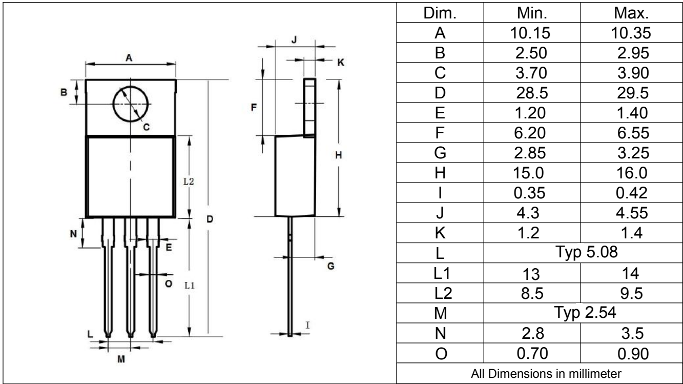
TO-220AB 封装尺寸 Package size
