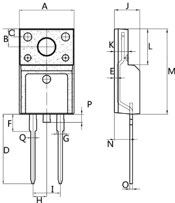
TO-220FAC 封装尺寸 Package size
