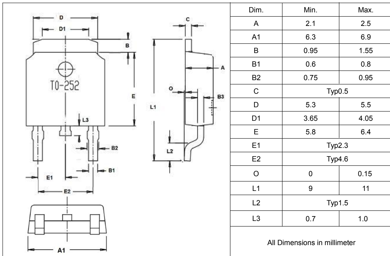
TO-252 封装尺寸 Package size
